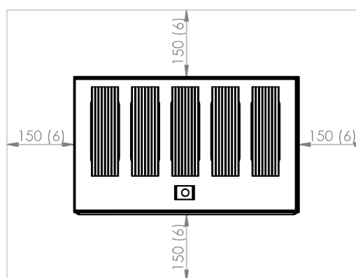
DIMMER 5 CHANNEL
