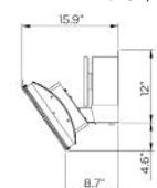
SIDE PROFILE (WITHOUT HEAT DEFLECTOR)
