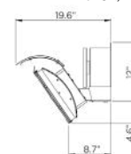
SIDE PROFILE (WITH HEAT DEFLECTOR)
