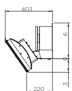
SIDE PROFILE (WITHOUT HEAT DEFLECTOR)
