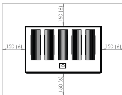
DIMMER 5 CHANNEL
