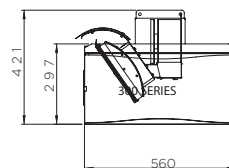
FRONT PROFILE (WITHOUT HEAT DEFLECTOR)
