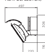
SIDE PROFILE (WITH HEAT DEFLECTOR)
