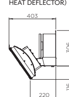
SIDE PROFILE (WITHOUT HEAT DEFLECTOR)
