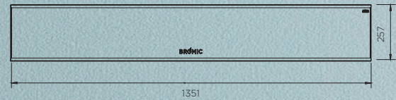
4500W Dimensions:
